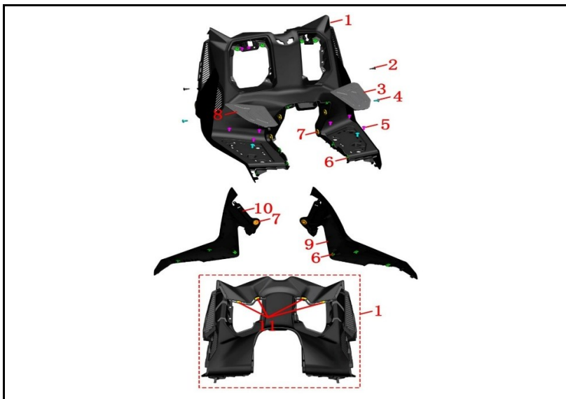
FIGURA N° 48: PANEL FRONTAL
