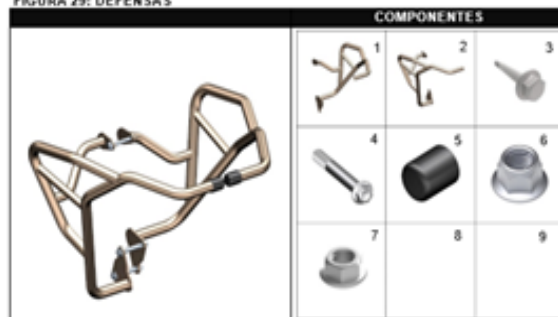
FIGURA 29: DEFENSA S
