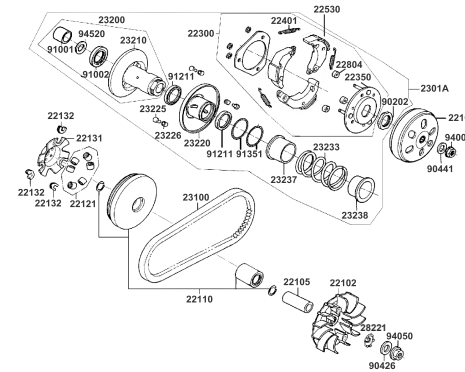
E05: CLUTCH CENTRIFUGO
